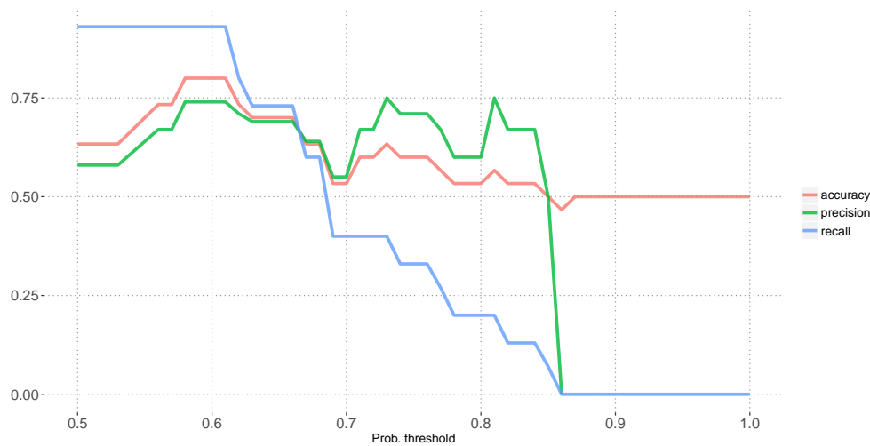
Figure 13: Precision, Recall and Accuracy of a binary classifier predicting protest images as we move the probability threshold used to transform SoftMax probabilities to a dichotomous variable
