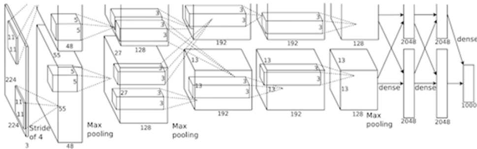
Figure 12: AlexNet architecture
